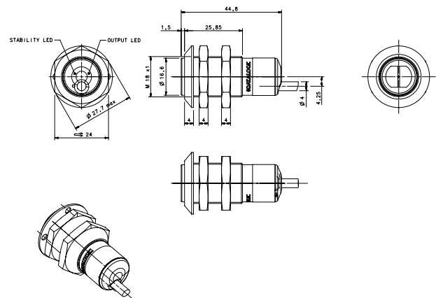
Cable version
